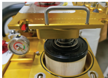
Top Loading Filter Design Allows for Quick, Clean Replacement
