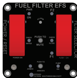
Remote Control Panel with Optional EFS (Electronic Filter Switching) Capability
